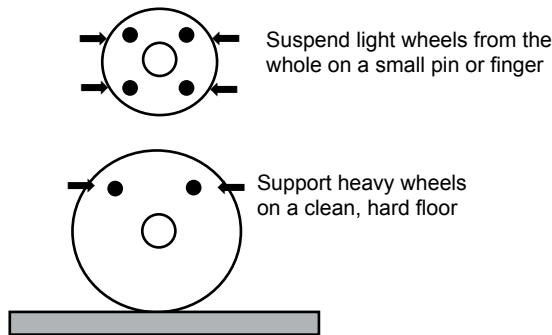
Figure 2 The Ring Test
