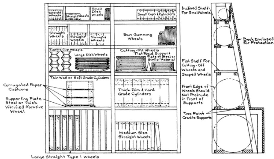
Figure 1 Proper Storage of Grinding Wheels
